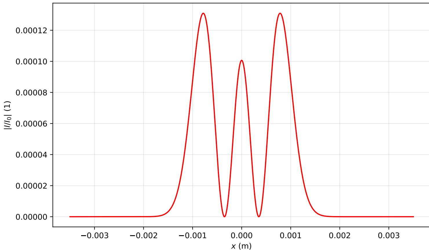
Intensity profile I(x, y = 0, z = 0.080)/I_0 , P_{in}=3.0P_{cr} , artificial time
